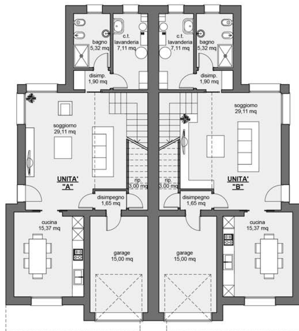
PIANO TERRA
