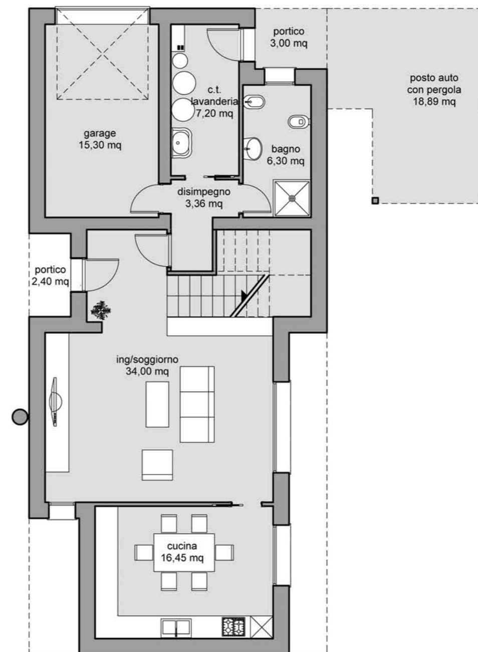
PIANO TERRA
